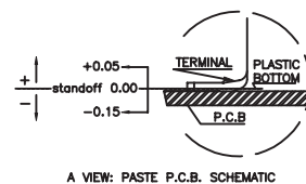
A VIEW: PASTE P.C.B. SCHEMATIC
