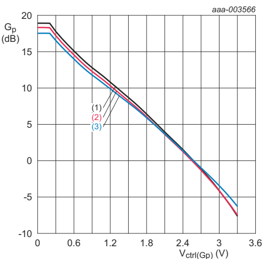
GS1 = HIGH; GS2 = LOW; V_{CC1} = 5\text{ V} ; V_{CC2} = 5\text{ V} ; f = 1950\text{ MHz} . (1) T_{amb} = -10\text{ }^{\circ}\text{C} (2) T_{amb} = +25\text{ }^{\circ}\text{C} (3) T_{amb} = +85\text{ }^{\circ}\text{C}
