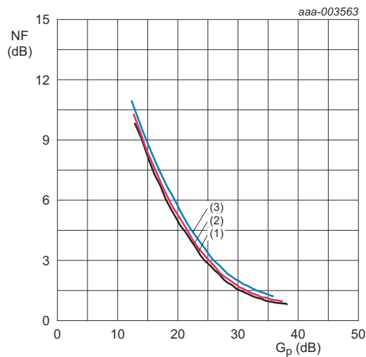
GS1 = LOW; GS2 = HIGH; V_{CC1} = 5\text{ V} ; V_{CC2} = 5\text{ V} ; f = 1950\text{ MHz} . (1) T_{amb} = -10\text{ }^{\circ}\text{C} (2) T_{amb} = +25\text{ }^{\circ}\text{C} (3) T_{amb} = +85\text{ }^{\circ}\text{C}
