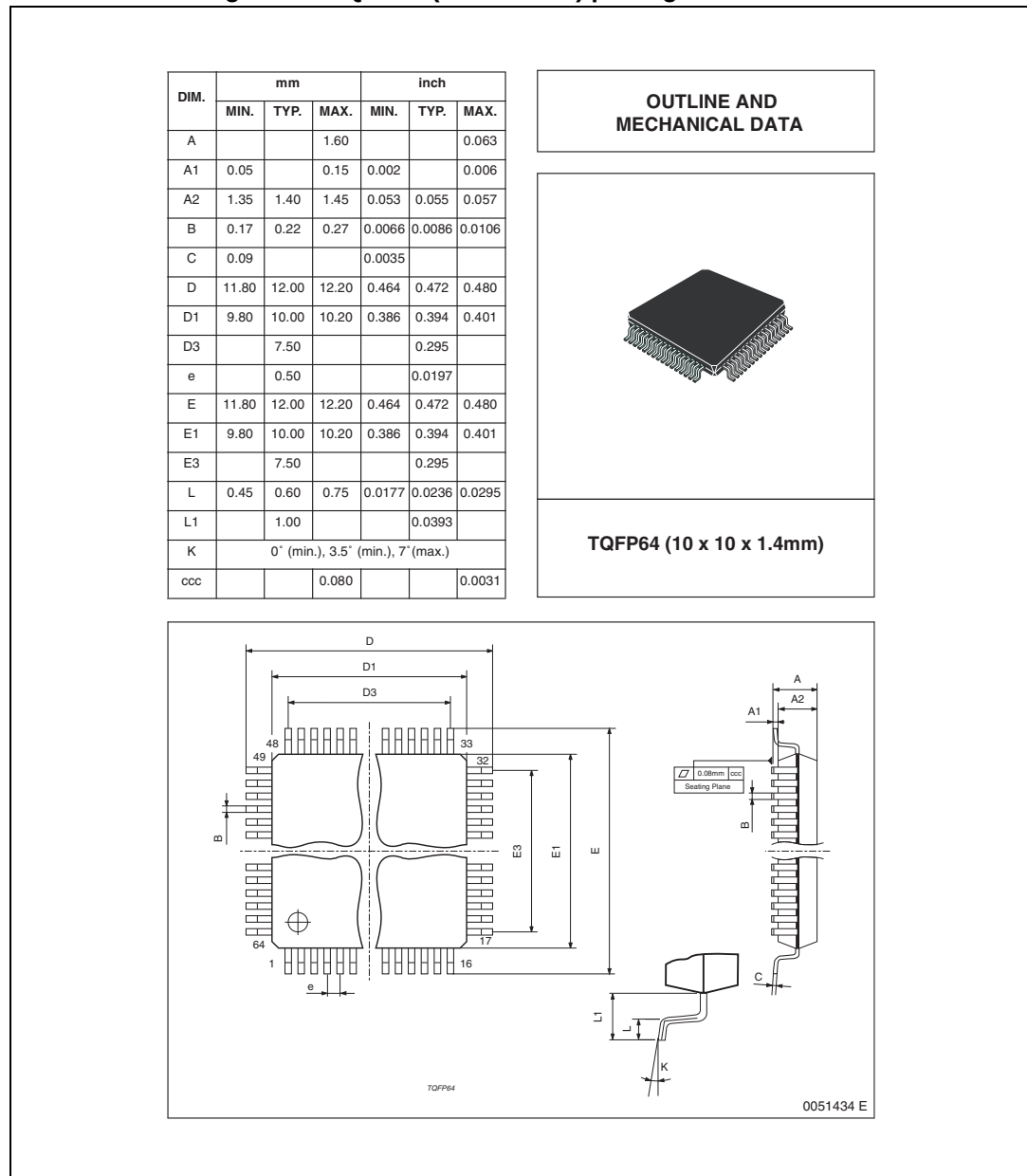
Figure 12. TQFP64 (10 x 10 mm) package dimensions
