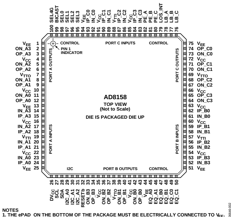
Figure 3. Pin Configuration
