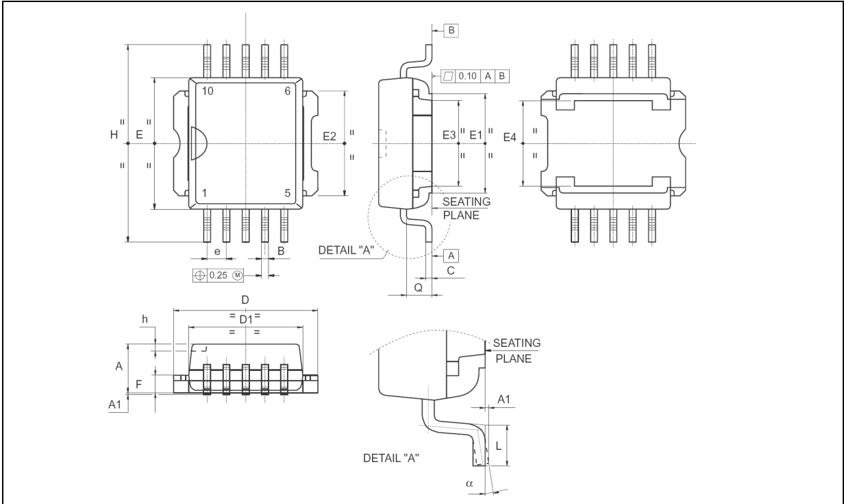
Figure 9. Package dimension
