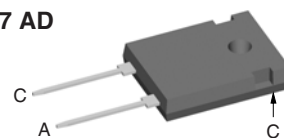
TO-247 AD
