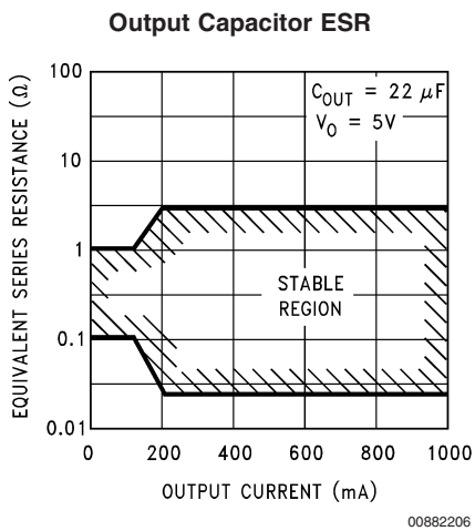
FIGURE 1. ESR Limits
