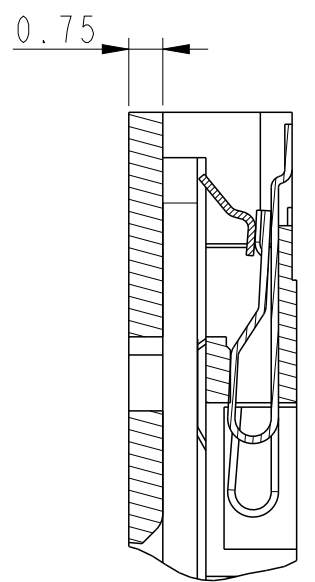
CARD SECTION B-B SCALE 6:1
