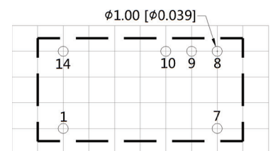
Top View PCB Layout
