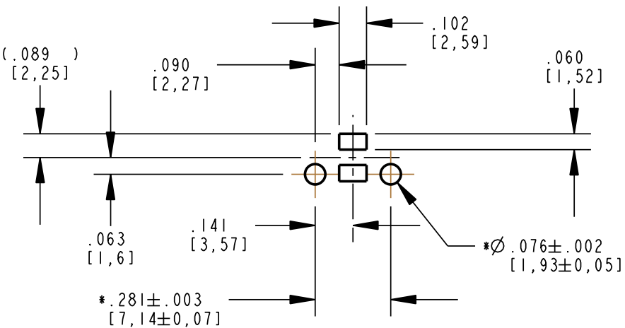
SOLDER PAD/HOLE LAYOUT FOR SINGLE COLOR
