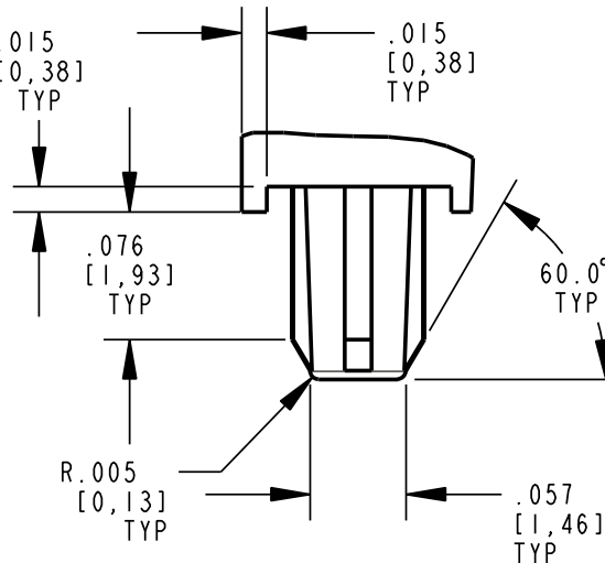
DETAIL B SCALE 8.000
