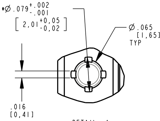
DETAIL A SCALE 8.000
