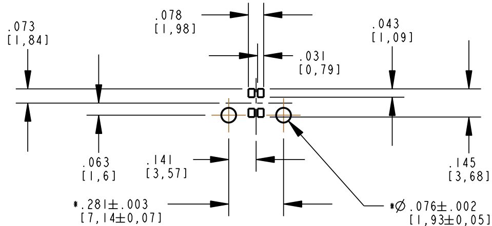
SOLDER PAD/HOLE LAYOUT FOR BI-COLOR
