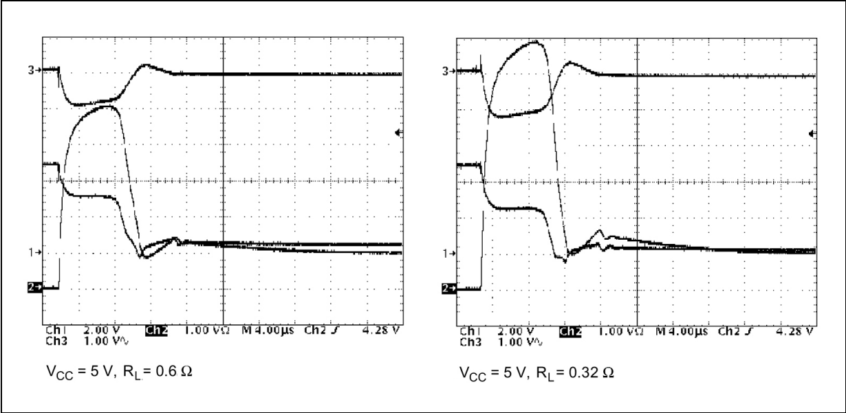
Figure 7. Switching waveforms
