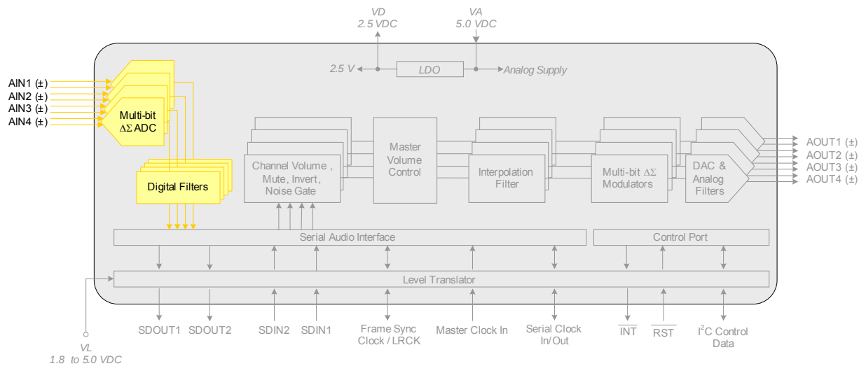
Figure 23. ADC Path
