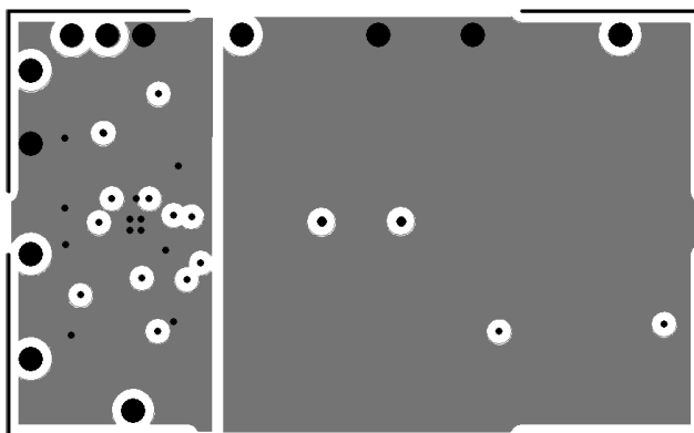
Figure 15. SP6136EB PCB Layout Bottom Side
