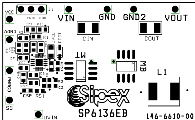
Figure 13. SP6136EB Component Placement
