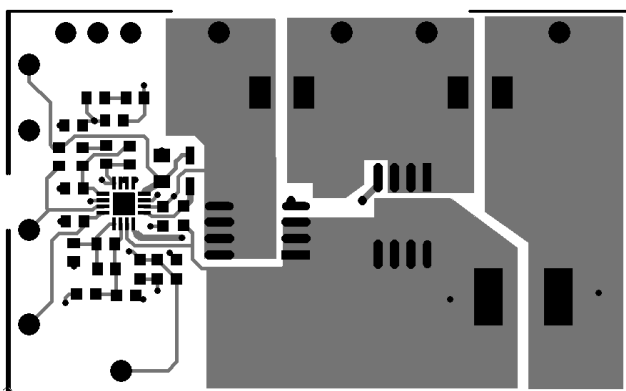
Figure 14. SP6136EB PCB Layout Top Side
