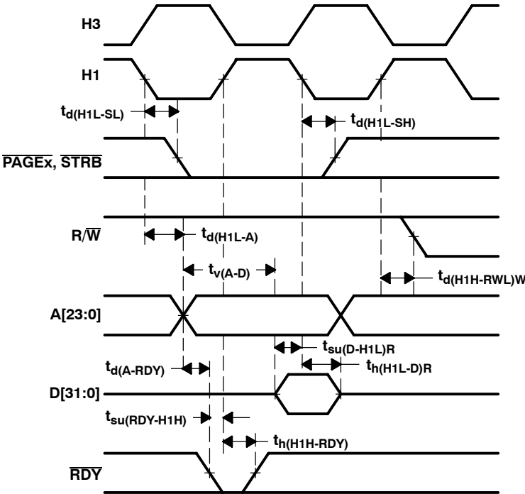
Figure 20. Timing for Memory ( \overline{\text{STRB}} = 0 and \overline{\text{PAGE}} = 0 ) Read
