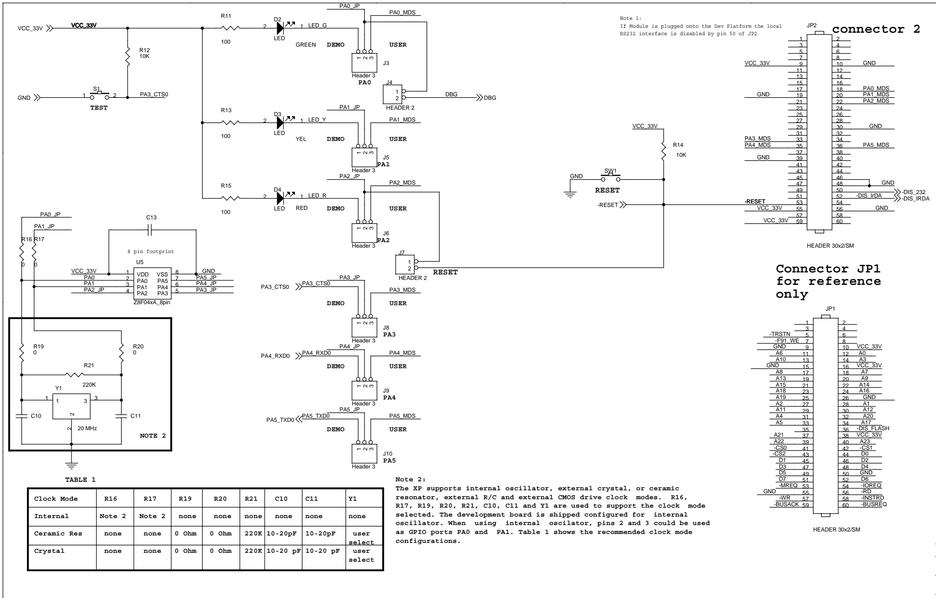
Figure 4. Schematic for Z8 Encore! XP F042A Series 8-Pin MCU Development Board
