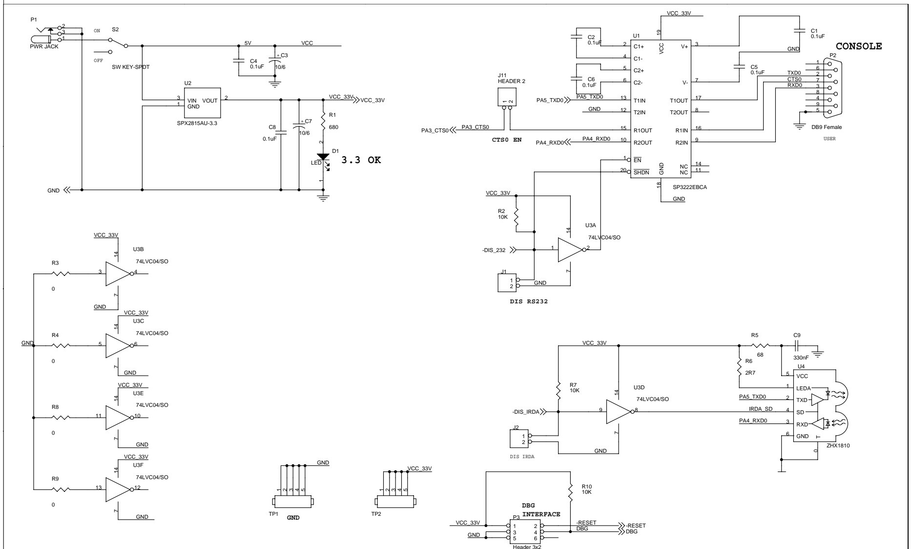
Figure 3. Schematic for Z8 Encore! XP F042A Series 8-Pin MCU Development Board
