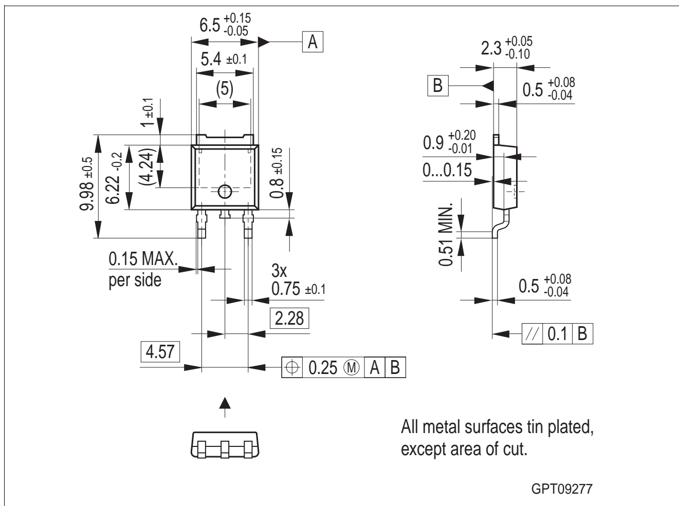
Figure 1 PG-TO252-3-11 (Plastic Dual Small Outline Package) (RoHS-Compliant)
