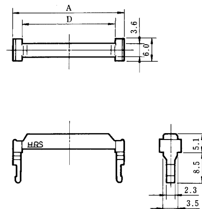
Clamp
