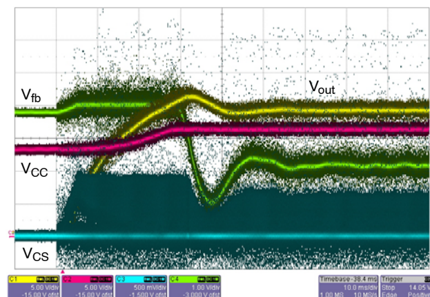
Figure 16. Startup Transient
