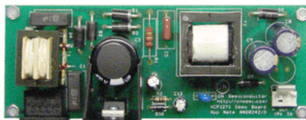
Figure 1. Evaluation Board Photo
