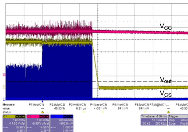
Figure 18. Short Circuit Protection is Activated When the Output Load Increases to about 100 W
