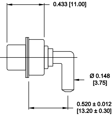
40 AMP POWER CONTACT
