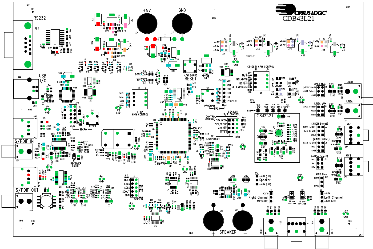
Figure 16. Silk Screen
