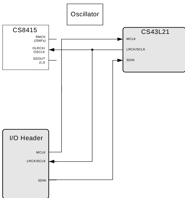
Figure 6. Routing 3
