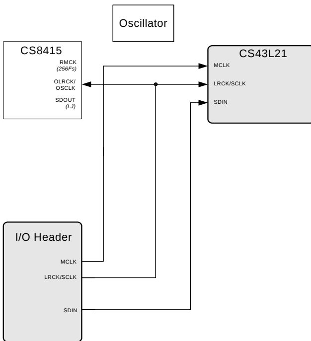
Figure 5. Routing 2
