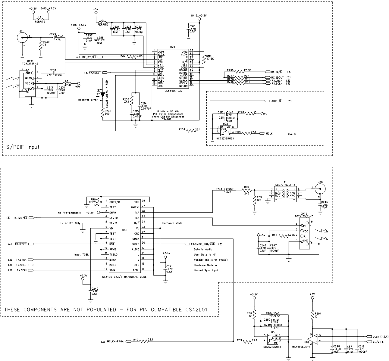
Figure 11. S/PDIF I/O (Schematic Sheet 2)
