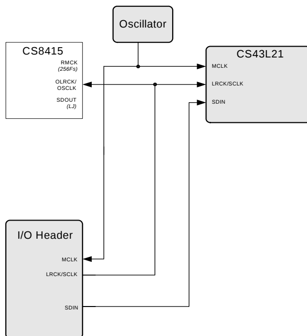
Figure 7. Routing 4
