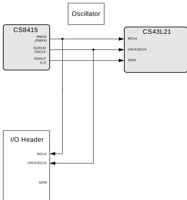
Figure 4. Routing 1
