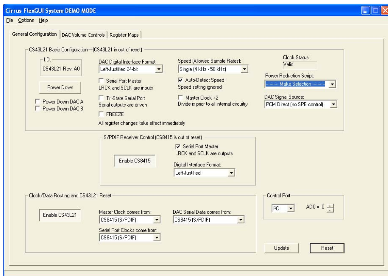
Figure 1. General Configuration Tab
