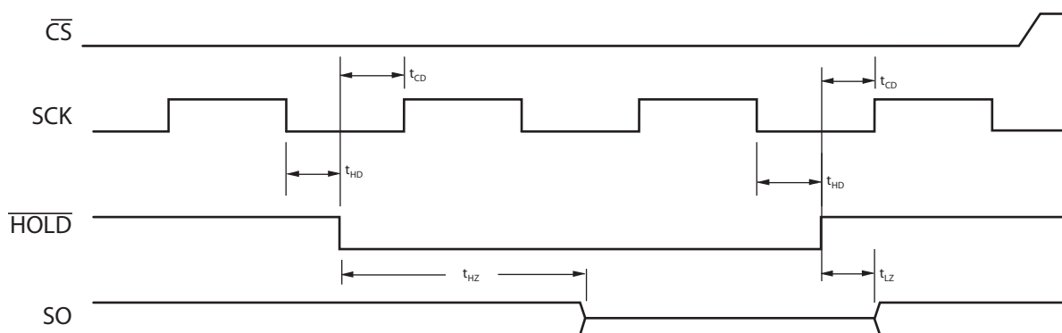
Figure 16 – \overline{HOLD} Timing
