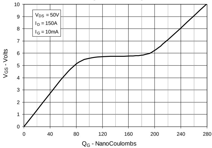
Fig. 9. Gate Charge
