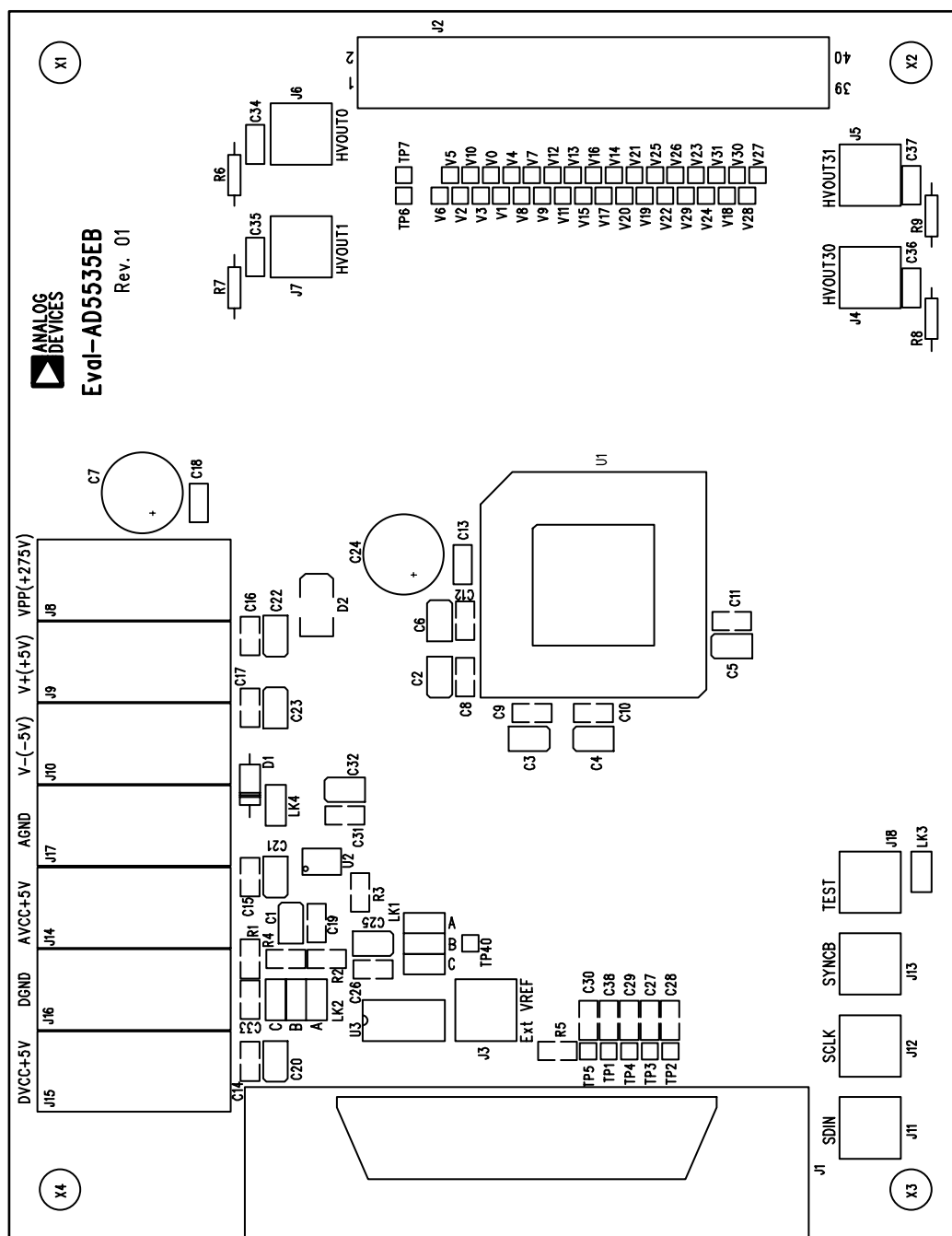
Figure 7. Component Placement Diagram
