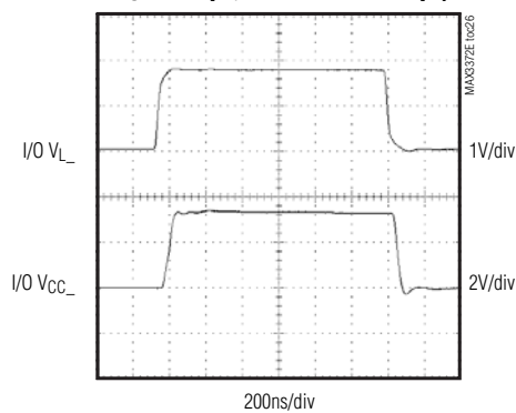
RAIL-TO-RAIL DRIVING (DRIVING I/O V_L , V_{\text{CC}} = +3.3\text{V} , V_L = +1.8\text{V} , C_{\text{LOAD}} = 15\text{pF} , DATA RATE = 8Mbps)
