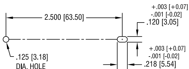
SUGGESTED MOUNTING DETAIL
