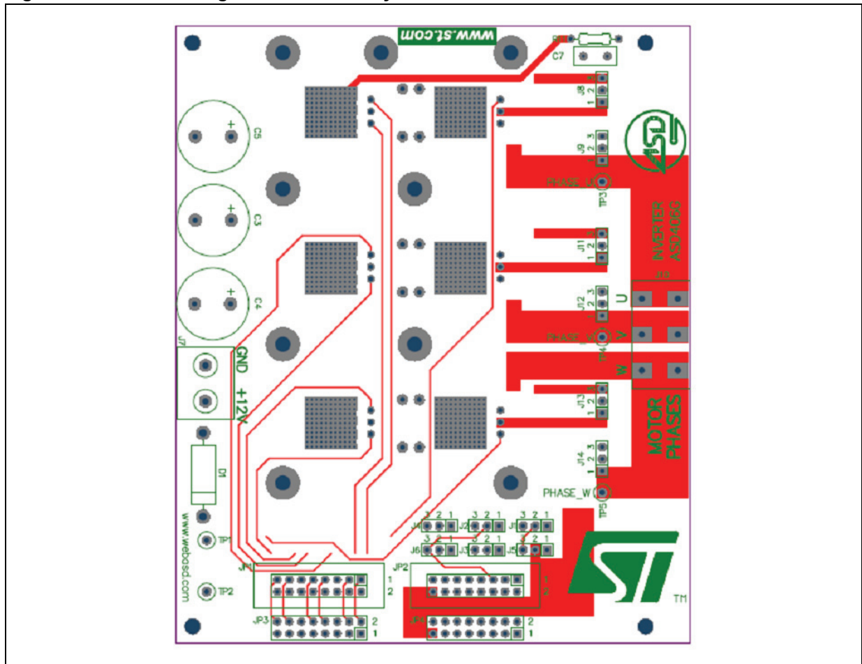
Figure 10. Inverter daughterboard front layout
