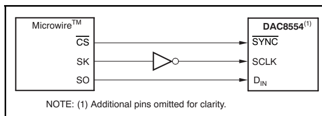
Figure 51. DAC8551 to Microwire Interface
