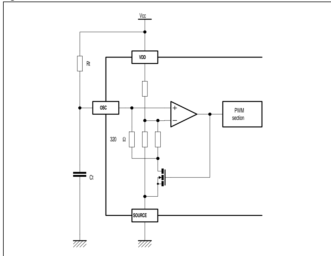
Figure 15. Oscillator Schematic
