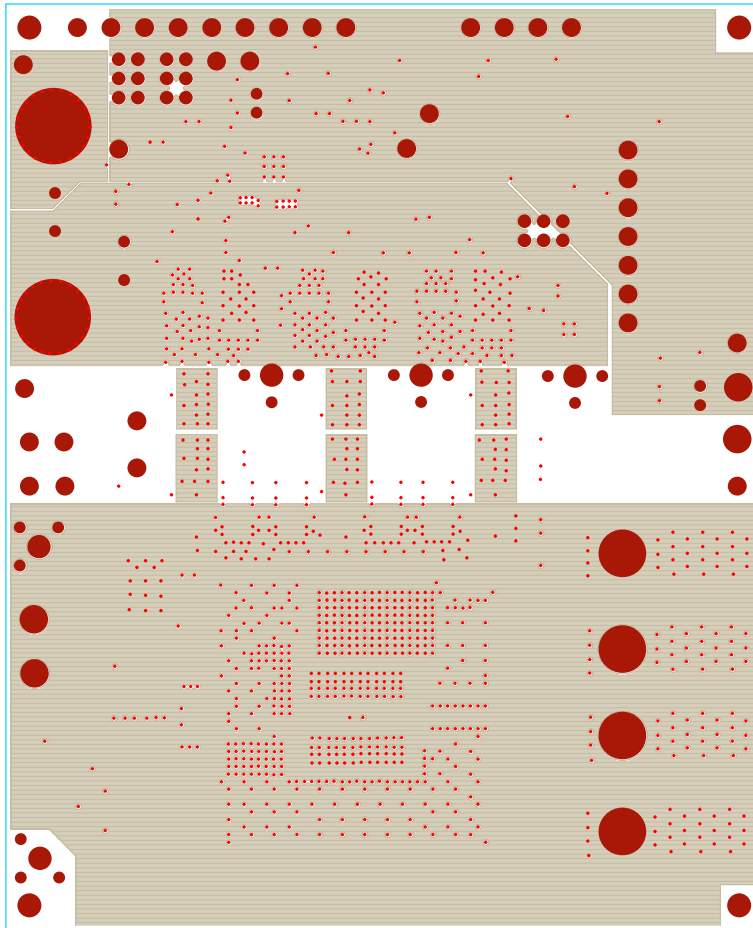
FIGURE 14. LAYER 6
