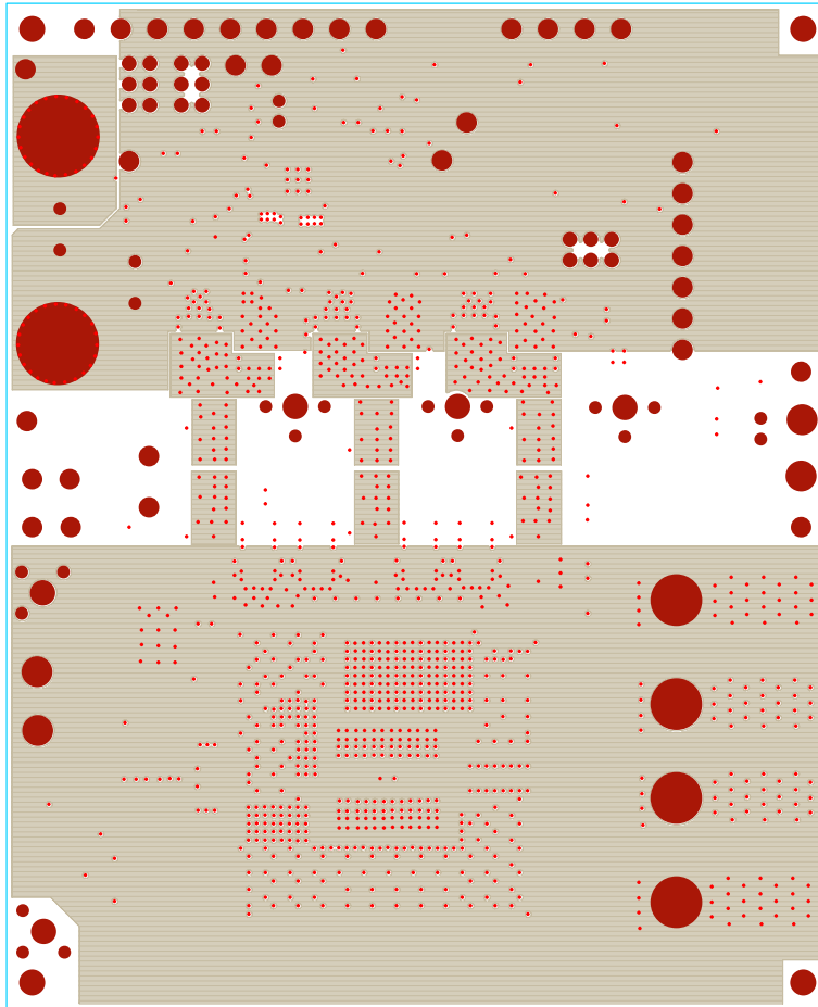
FIGURE 12. LAYER 4
