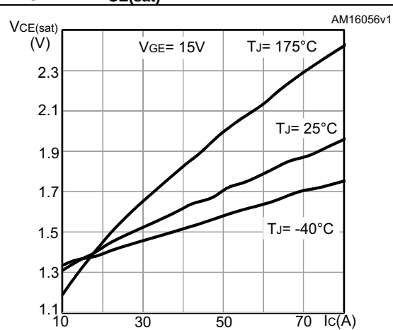
Figure 9. V_{CE(sat)} vs. collector current
