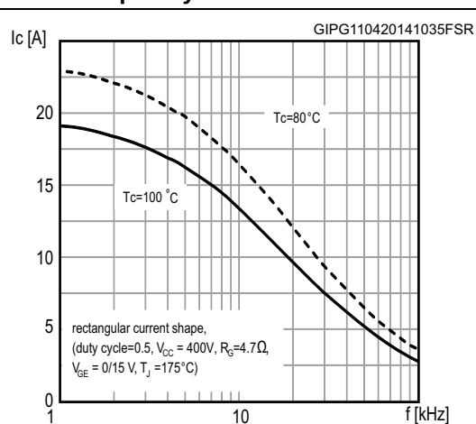
Figure 11. Collector current vs. switching frequency for TO-3PF
