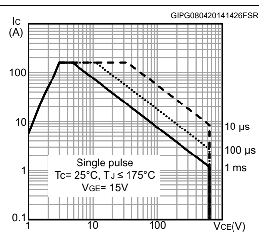
Figure 13. Forward bias safe operating area for TO-3PF
