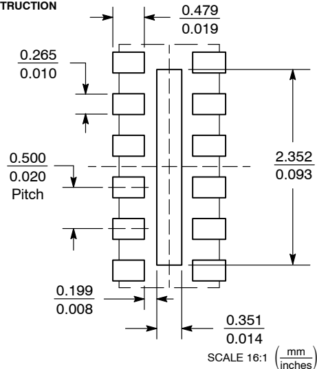
DETAIL A OPTIONAL CONSTRUCTION
