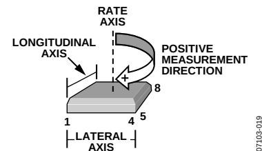
Figure 13. Rate Signal Increases with Clockwise Rotation
