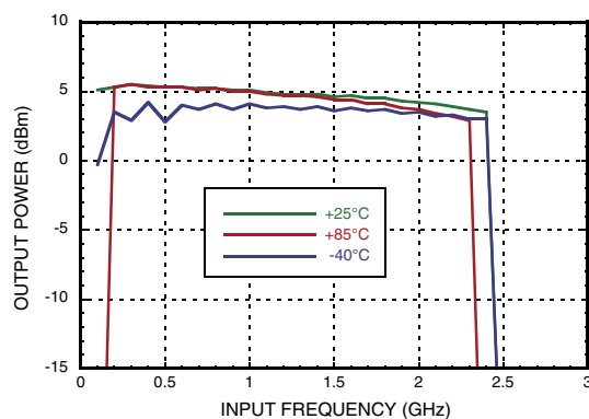
Pout Divide-by-3 vs. Temperature [1] , (Single-Ended)
