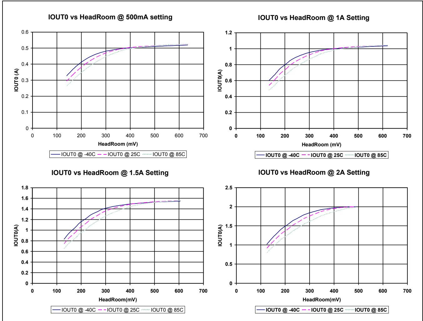
Figure 1-1. Typical IOUT0 Current vs Headroom
