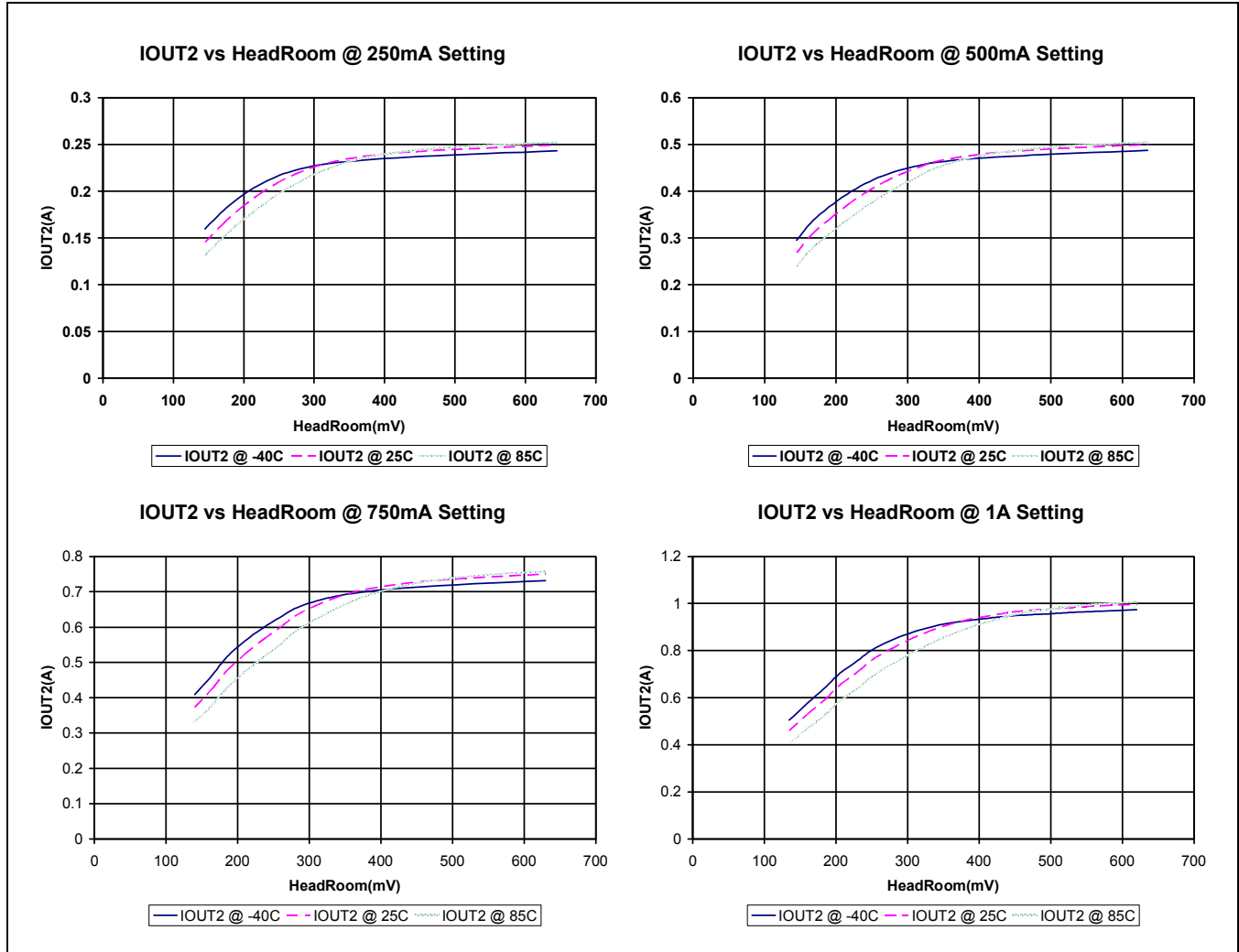
Figure 1-3. Typical IOUT2 Current vs Headroom
