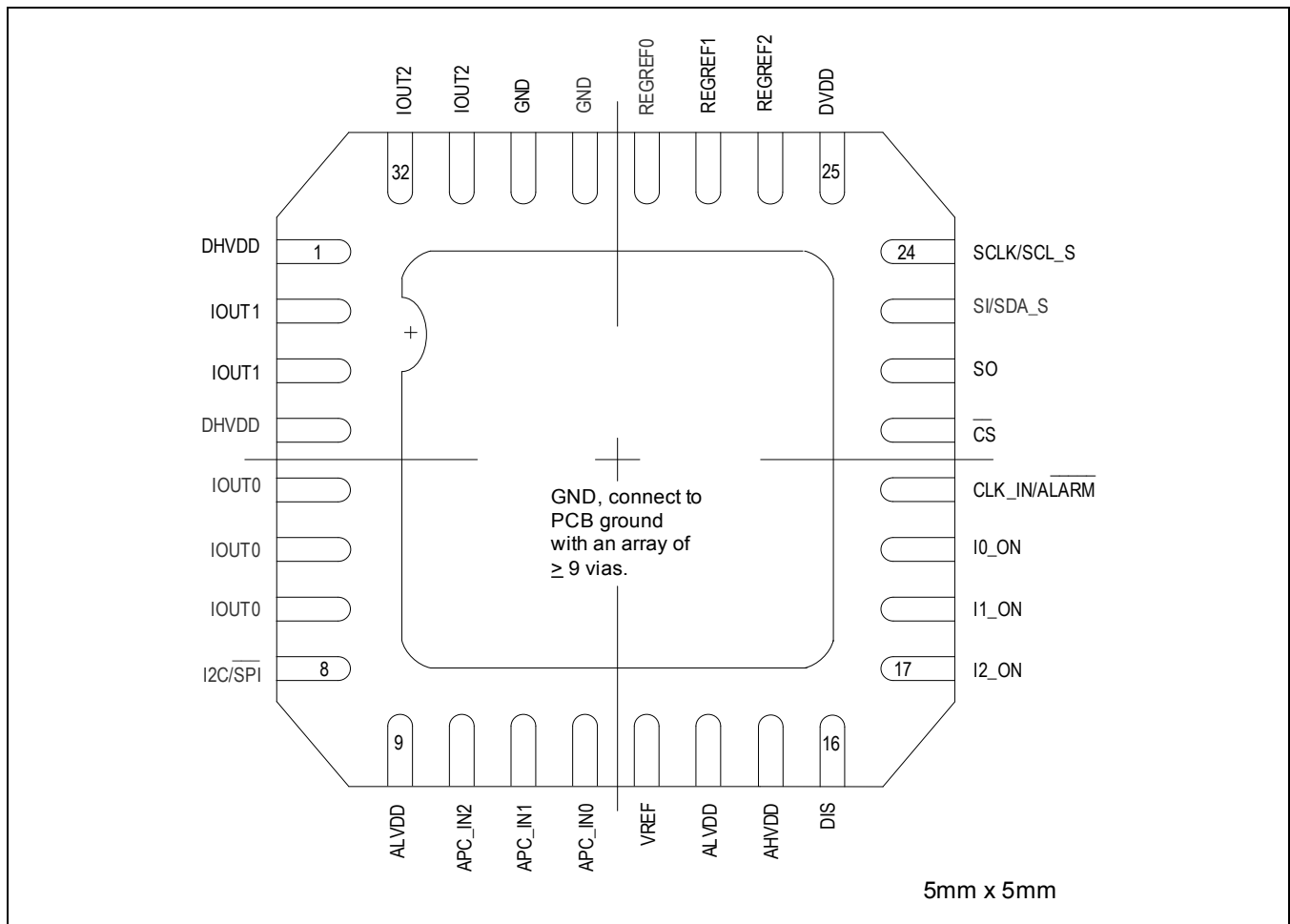
Figure 1-10. M08886 Pinout
