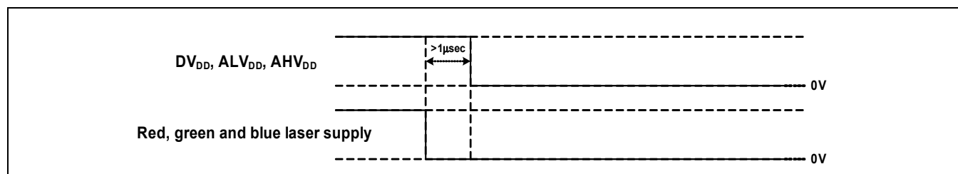
Figure 2-7. Power-Down
