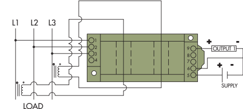
CR6240 CR6241 2 element - 3 Wire, 4 - 20 mADC Output shown with external current transformer
