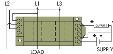
CR6240 CR6241 2 element - 3 Wire, 4 - 20 mADC output
