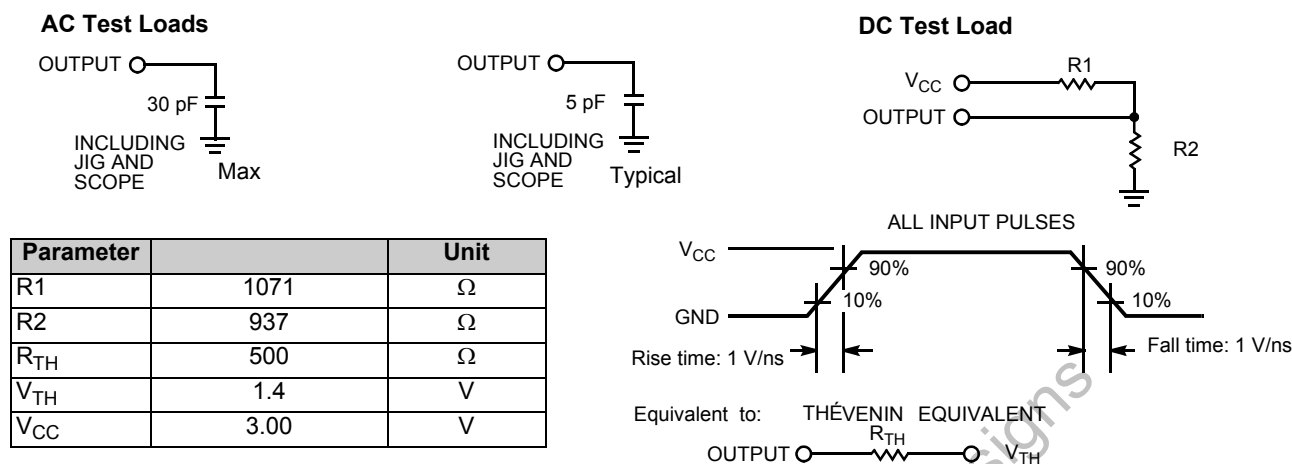
Figure 17. AC Test Loads and Waveforms for Digital Pins
