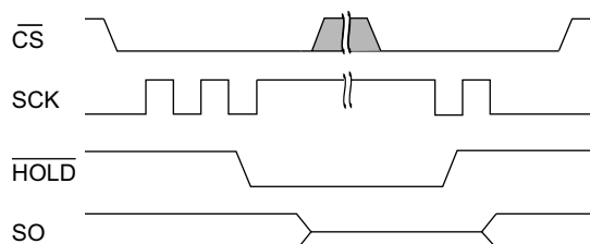
Figure 28. HOLD Operation
