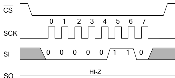
Figure 10. WREN Instruction
