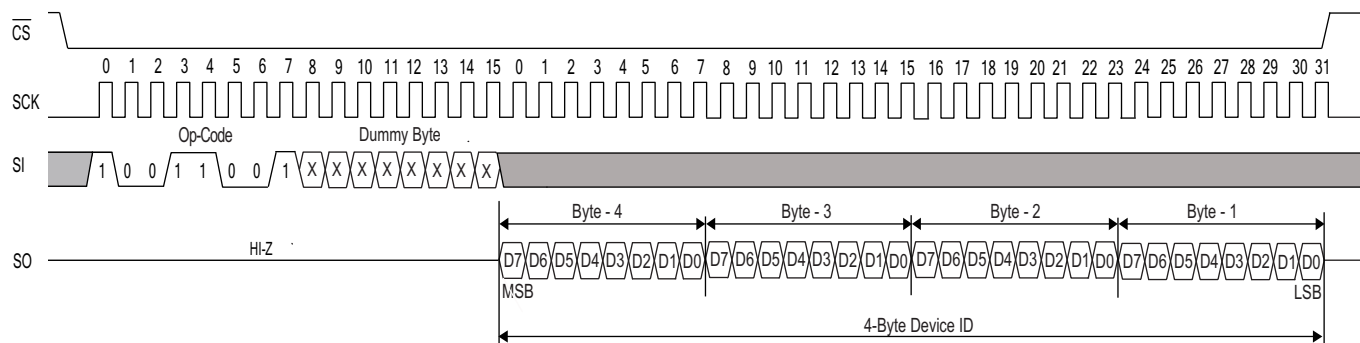
Figure 27. FAST_RDID instruction
