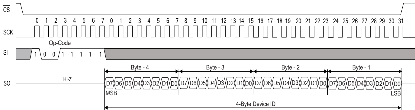
Figure 26. RDID instruction
