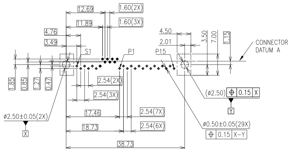
RECOMMENDED PCB LAYOUT PCB THICKNESS 1.50 TO 2.50
