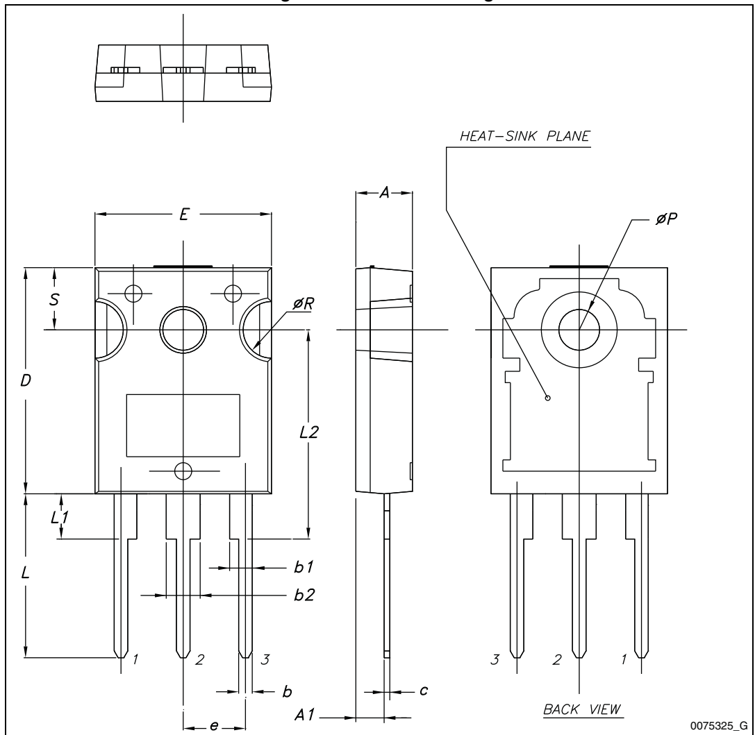
Figure 32. TO-247 drawing
