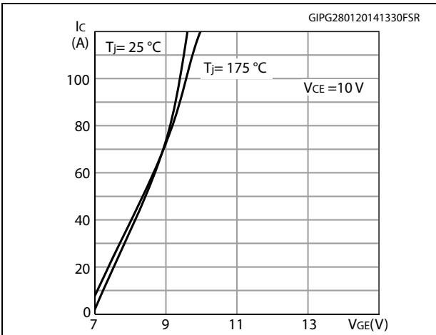
Figure 10. Transfer characteristics
