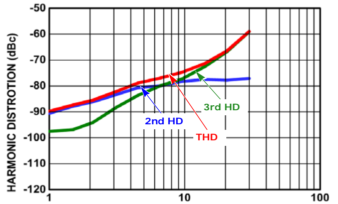
FIGURE 4. 4MHz HARMONIC DISTORTION vs OUTPUT SWING
