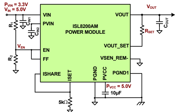
FIGURE 21. 3.3V OPERATION
