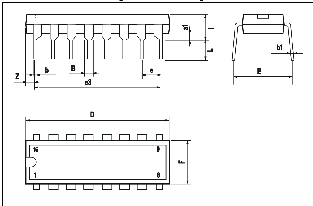
Figure 21. DIP16 drawing
