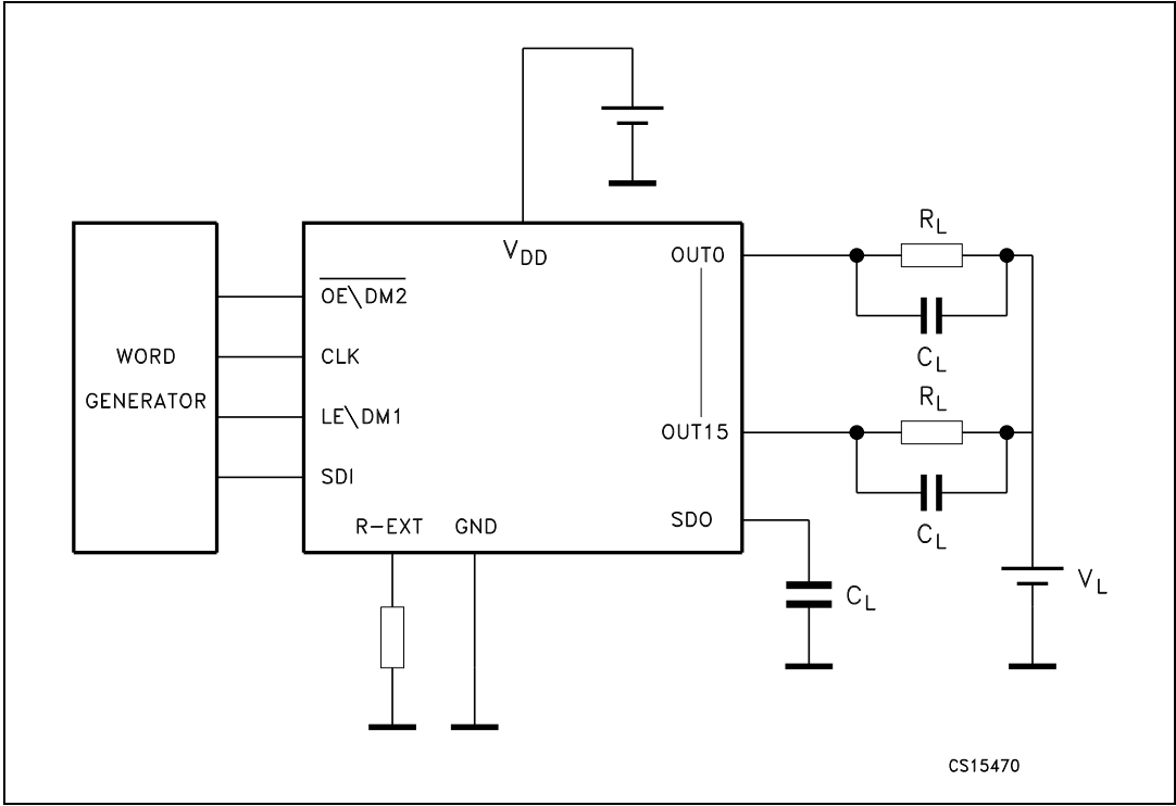
Figure 15. AC characteristics
