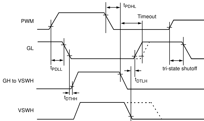
Figure 4. Timing Diagram
