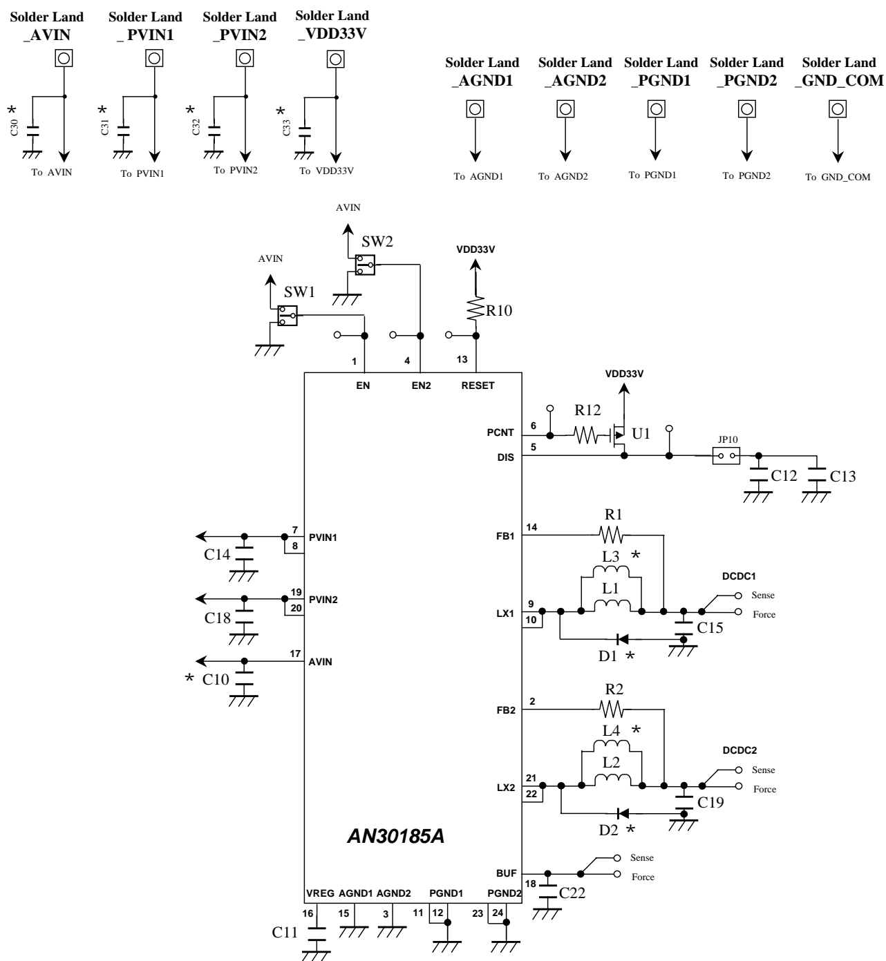
Figure 5. Evaluation Board Schematic
