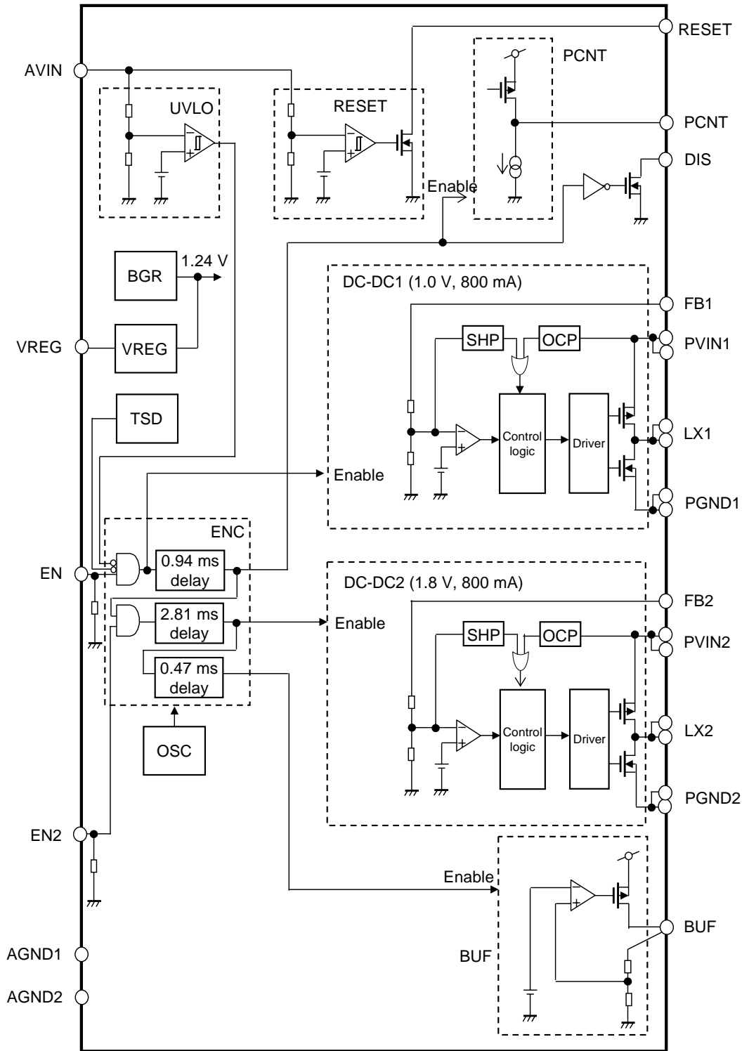
Figure 1. Block Diagram
