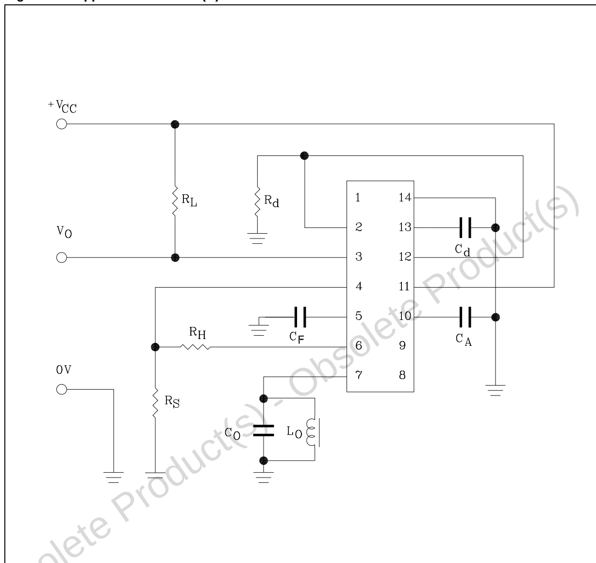
Figure 11. Application Scheme (C)
