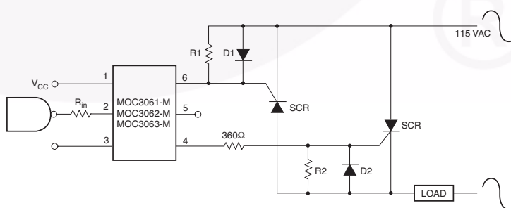
Figure 11. Inverse-Parallel SCR Driver Circuit
