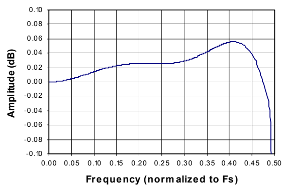
Figure 32. DSM Passband Ripple
