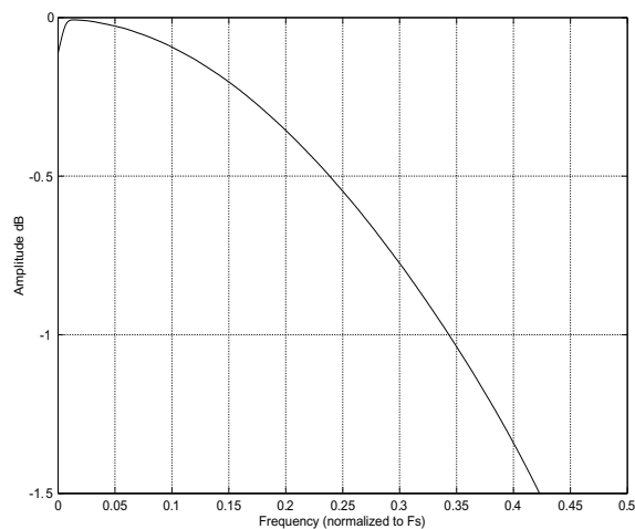
Figure 44. QSM Passband Ripple
