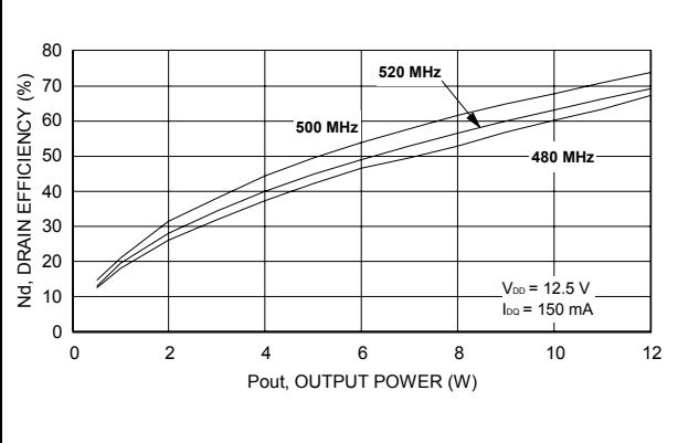
Figure 8. Drain efficiency vs. output power
