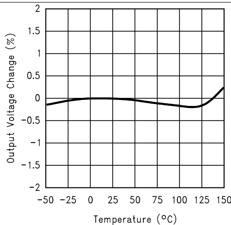
Figure 6. Temperature Stability
