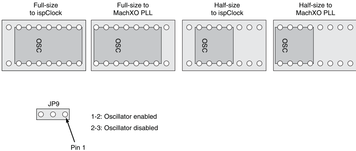
Figure 6. Oscillator Positions
